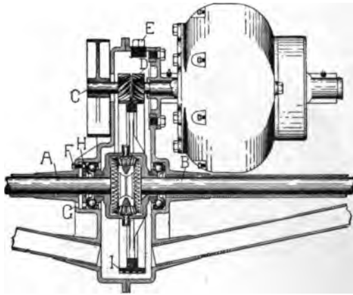
FIG. 297.—Plan Diagram of Single Motor Attached to Rear Axle Through "Herring-bone" Single Reducing Gears. A is the left-hand section of the divided rear axle; B, the right-hand section of the rear axle; C, the brake drum; D, the spiral pinion on the motor shaft driving the worm gear, I, on the differential; E, plug for greasing gears; F, set screw for locking ball race; G, slot for wrench to adjust threaded ring, H, against ball bearings.
